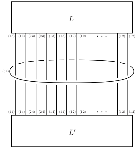
(a) By isotopically moving the trivial sheet
